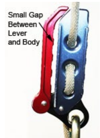
Fig. 7 Click-To-Neutral Position
