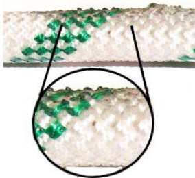
Melted / Glossy / Glazed Strands
