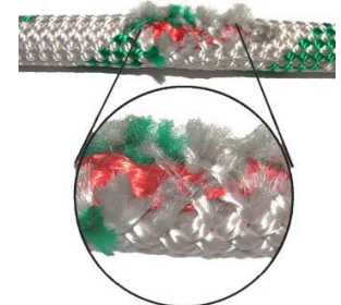
Rope with Warning Center Exposed
