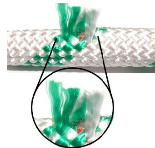
Rope with Broken or Cut Strands
