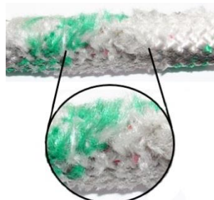
Rope with Excessive Abrasion Wear
