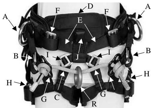
Model 17905 (front view)
